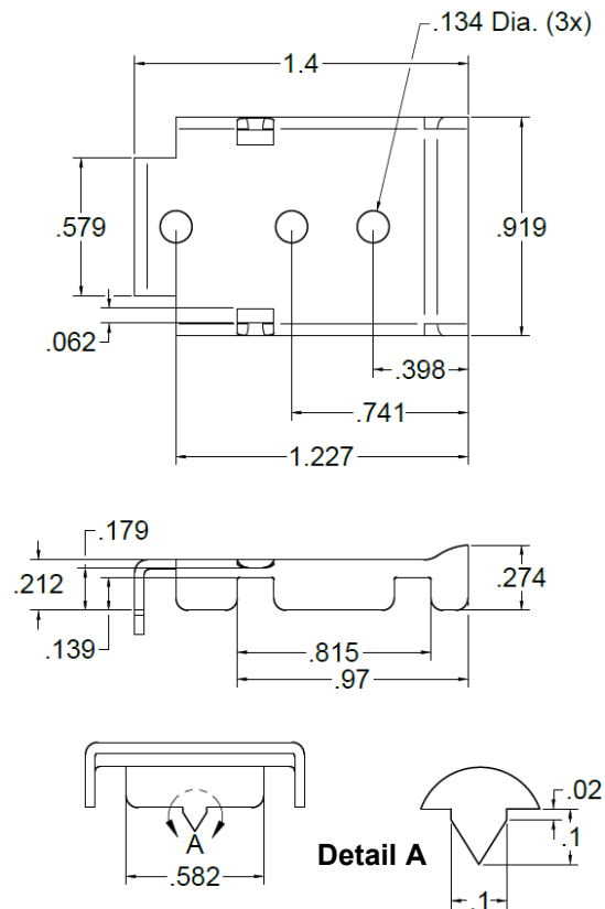
5050-P Bracket
