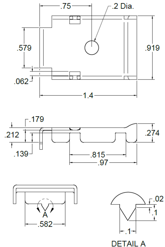
5051 Bracket
